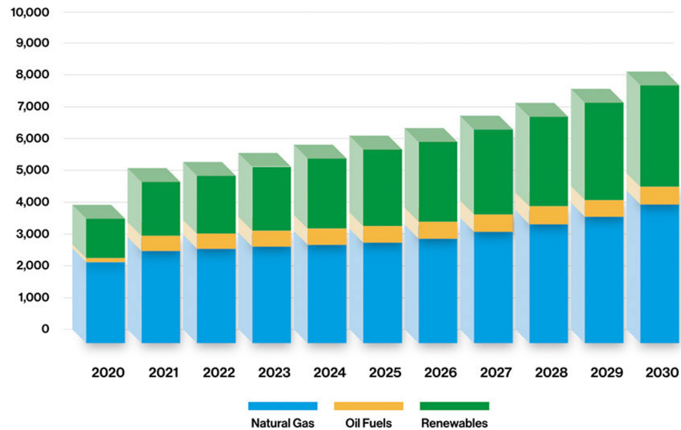
Installed Capacity - Power Capacity by Fuel, MW
